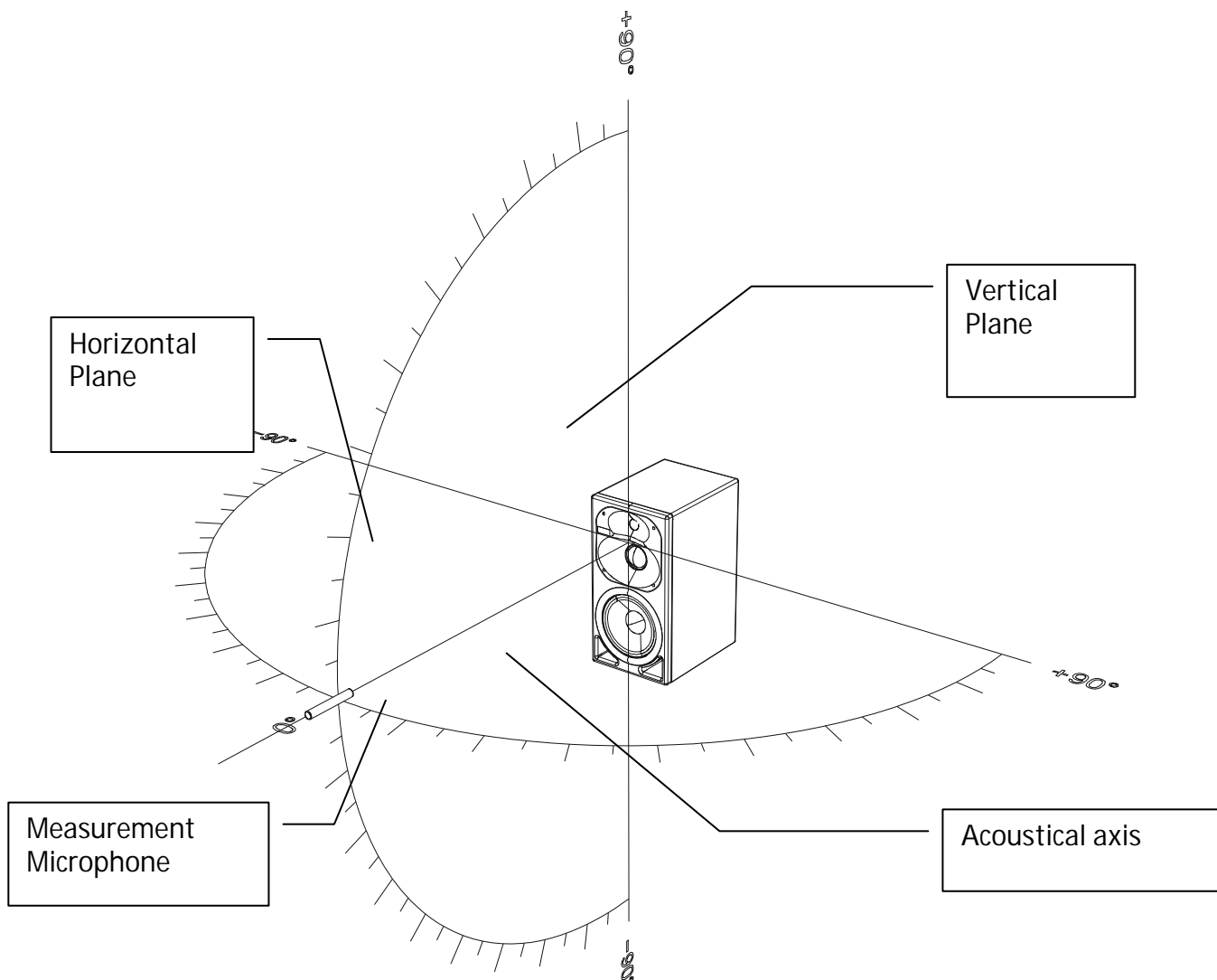
Setup for measuring a loudspeaker's radiation pattern
