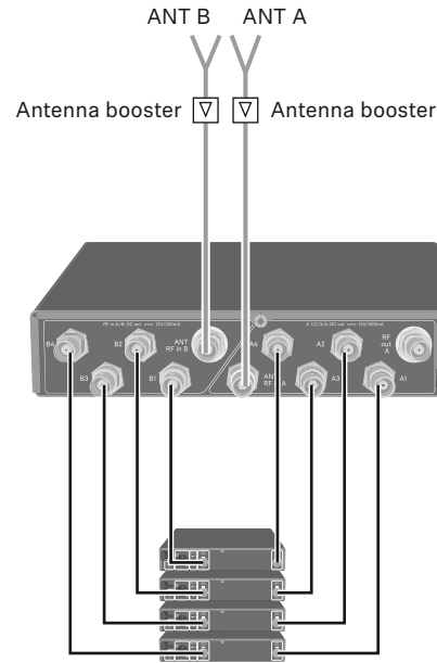
A: Two antennas supplying a 4-channel system
