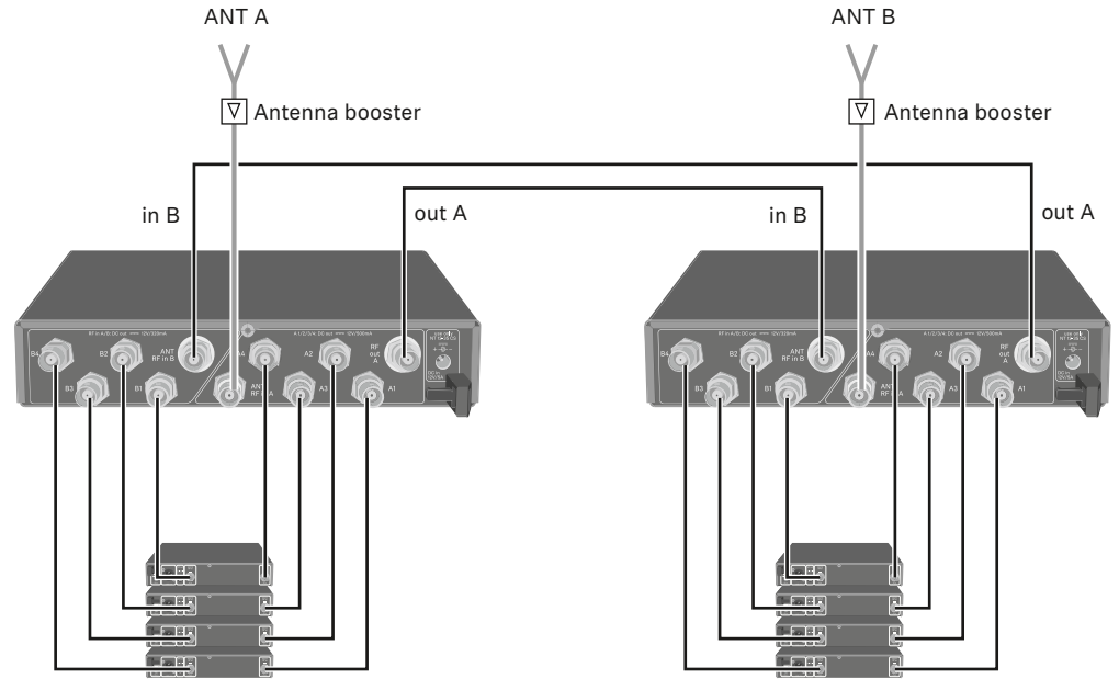
B: Linking two 4-channel systems
