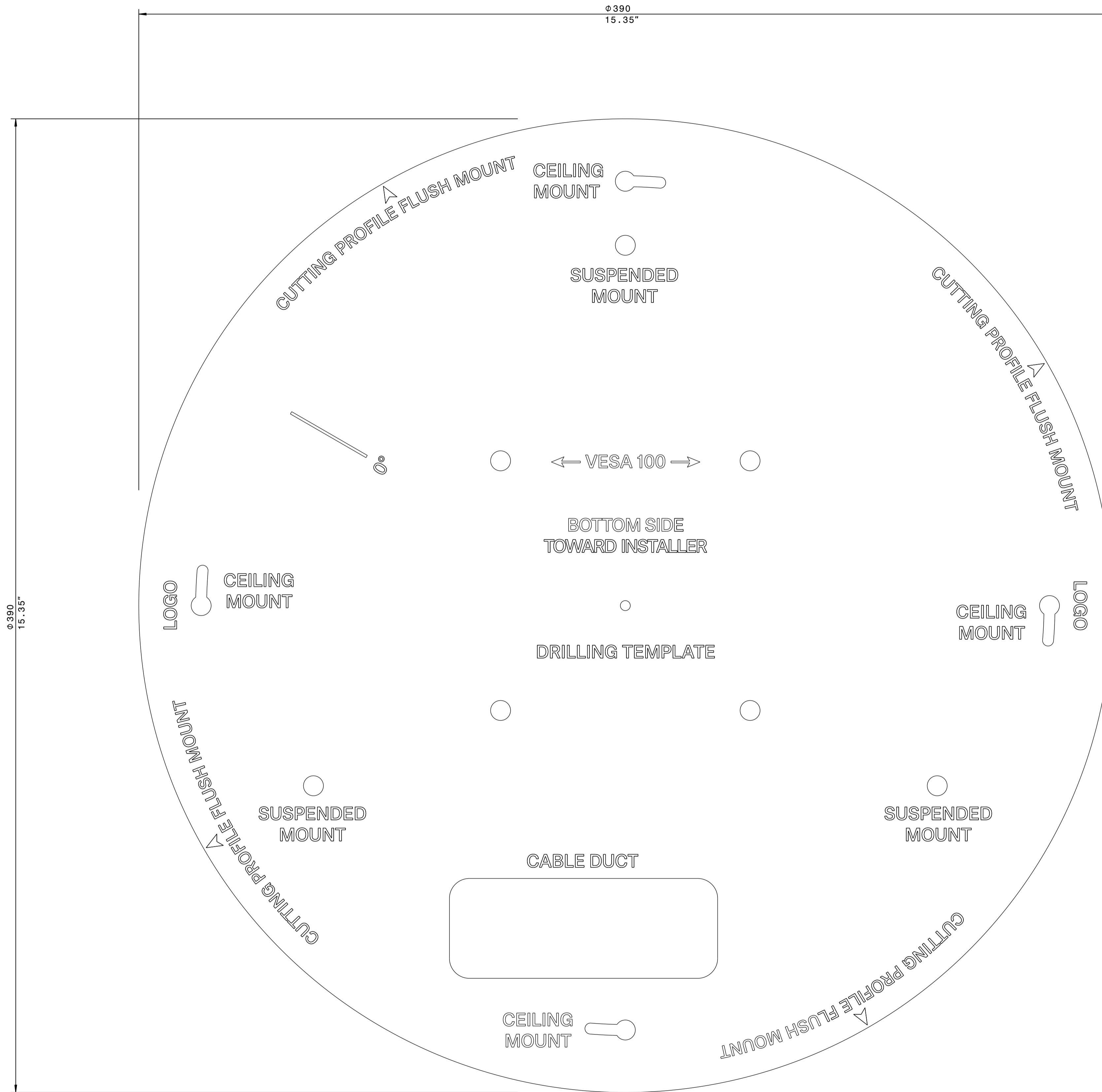
594561 drilling template TCC M Please check the outer diameter after printing vertical and horizontal to avoid any possible distortion. Minimum plotter paper width: A1 590mm, ANSI D 22" or ARCH D 24"
